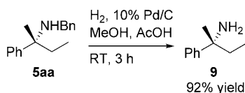
Scheme 3. Representative example for the selective deprotection of C-tertiary benzylamines.
