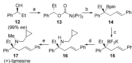
Scheme 5. Synthesis of (+)-igmesine. Reagents and conditions: a) i\text{Pr}_2\text{NCOCl} (1.05 equiv), \text{NEt}_3 (1.1 equiv), \text{CH}_2\text{Cl}_2 , reflux, 24 h, 92%; b) \text{sec} -butyllithium (1.1 equiv), -78^\circ\text{C} , 20 min; then cinnamyl boronic acid pinacol ester (1.2 equiv), -78^\circ\text{C} , 1 h; then 1 M \text{MgBr}_2 in MeOH (1.2 equiv), -78^\circ\text{C} , 10 min, then RT, 16 h; then 1 M aq \text{KH}_2\text{PO}_4 , 92%; c) 4.5 M aq \text{KHF}_2 (2.5 equiv), MeOH, RT, 30 min, evaporation; then 50% aq MeOH, 10 min and evaporation (5 \times ), 98%; d) \text{SiCl}_4 , (2 equiv), DCE, RT, 1 h; c\text{PrCH}_2\text{N}_3 (2 equiv), 80^\circ\text{C} , 30 min; then 2 M aq NaOH, RT, 1 h, 56%; e) 37% aq \text{CH}_2\text{O} , \text{NaHB}(\text{OAc})_3 , DCE, RT, 16 h, 99%. [18]
